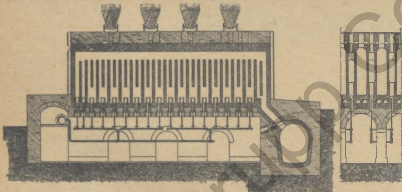
Otto-Unterbrenner-Öfen.
