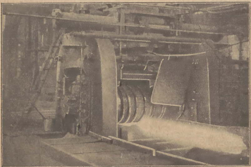
Blockwalze
