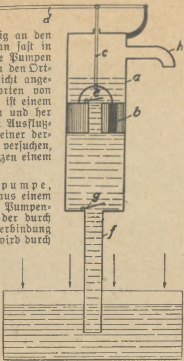
Fig. 1: Saugpumpe
