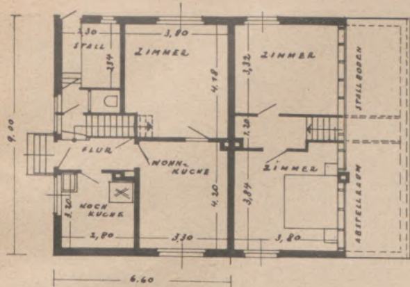
Bauart I Erdgeschoss
