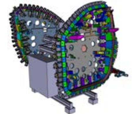
Double frame with application plates
