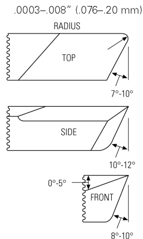
Figure 1: Lathe Tool
