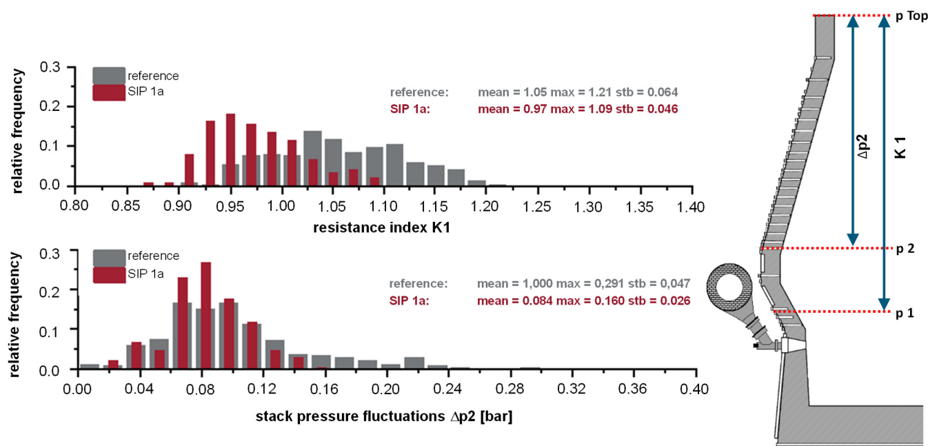
Figure 6. Comparison of the relative frequency distributions for the calculated resistance index K1 and the measured delta p values between the reference phase 1 and the SIP evaluation period 1a.
