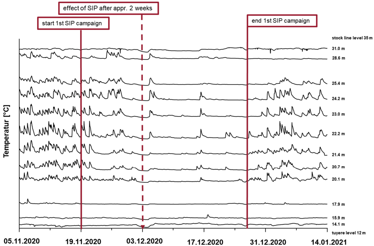
Figure 5. Schwelgern BF 1, wall temperatures above the tuyere level at one vertical measure line (line 5) during the first SIP campaign.
