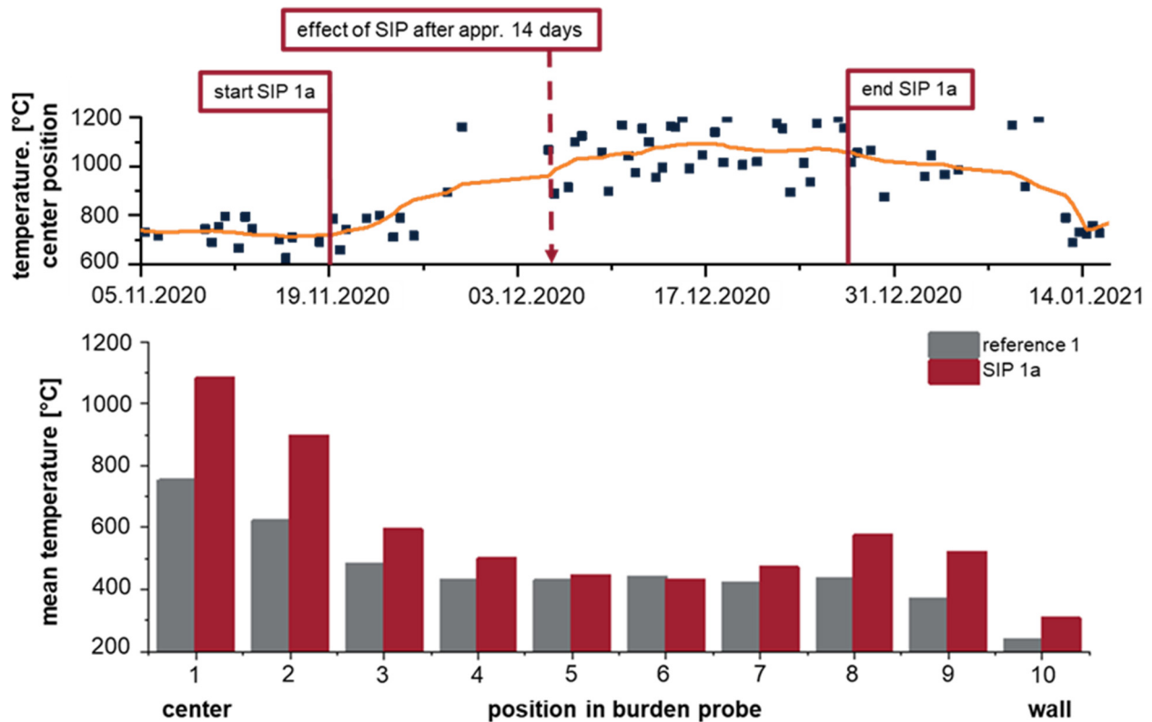
Figure 4. Schwelgern BF 1 in-burden probe (approx. 2 m below stock line level) temperature measurements, without and with SIP at the time of the first campaign. The top image shows development of the blast furnace center temperatures as measured with the in-burden probe, without and with SIP at the time of the first campaign.
