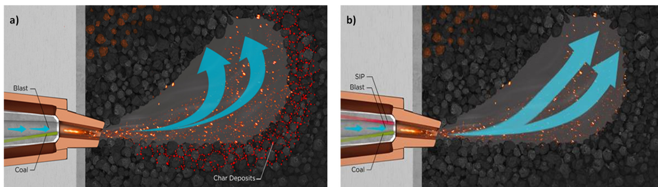
Figure 2. Conditions in the raceway and surrounding coke area a) without SIP, b) with SIP.
