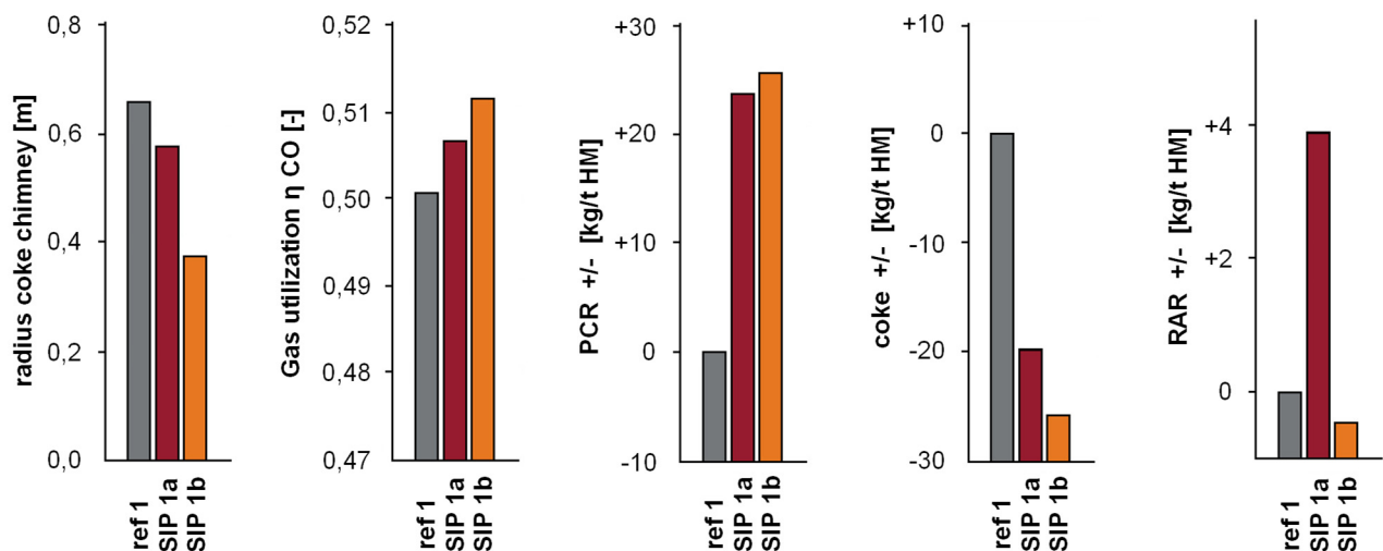
Figure 8. Comparison of average values of reference period 1 with SIP evaluation periods 1a and 1b.
